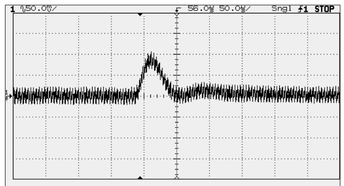
Output Voltage Response to Step Load (25.5A, +17.5A load step, di/dt = 1A/\mu s , T_{amb}=25C , V_{in}=48V )
