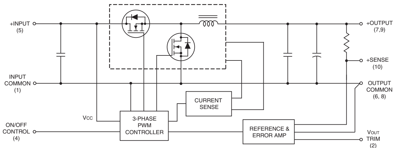
Figure 1. Simplified Schematic
