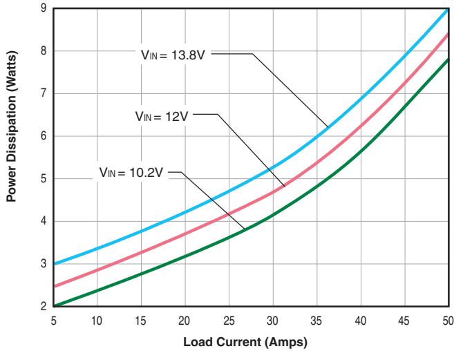
LQN-1.5/50-D12 Internal Power Dissipation vs. Load Current
