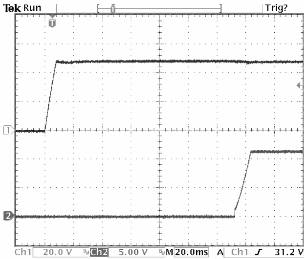
Figure 9 Ch3: En; Ch2: Vout V_{in}=48V, I_o=15A, C_o=3000\mu F
