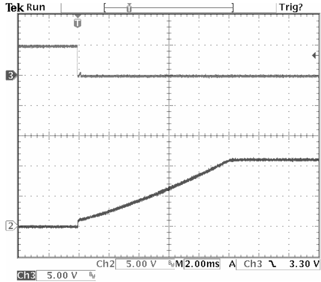
Figure 10 Ch3: Vin; Ch2: Vout V_{in}=48V, I_o=15A, C_o=3000\mu F
