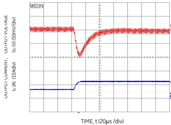
Figure 34. Transient Response to Dynamic Load Change from 50% to 100% at 12V in , C_{out}=5\times 47\mu\text{F} , C_{Tune}=1500\text{pF} & RTune-330ohms
