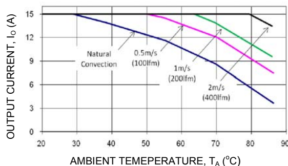
Figure 16. Output Current Derating for the Module with Heatplate; Airflow in the Transverse Direction from V_{out}(-) to V_{out}(+) ; V_{IN} = 48V , V_O = 5.0V .
