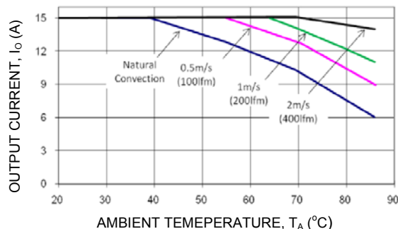
Figure 17. Output Current Derating for the Open Frame Module; Airflow in the Transverse Direction from V_{out}(-) to V_{out}(+) ; V_{IN} = 24V , V_O = 5.0V .
