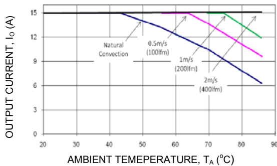
Figure 18. Output Current Derating for the Module with Heatplate; Airflow in the Transverse Direction from V_{out}(-) to V_{out}(+) ; V_{IN}=24V , V_O=5.0V .
