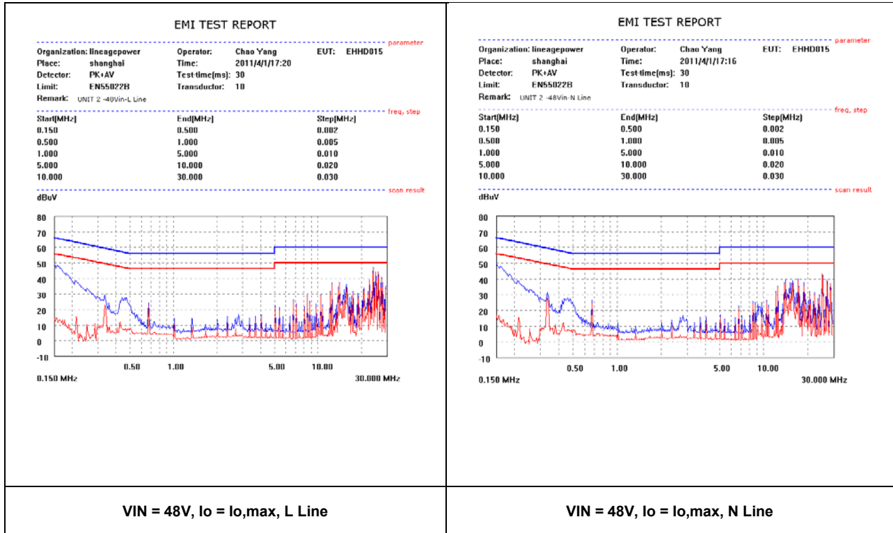
Figure 26. EMC Considerations
