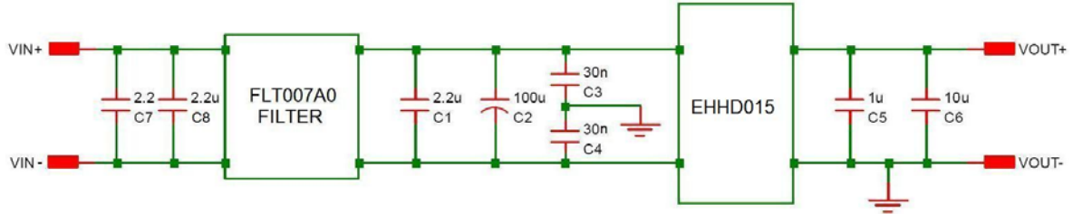
Figure 26. EMC Considerations
