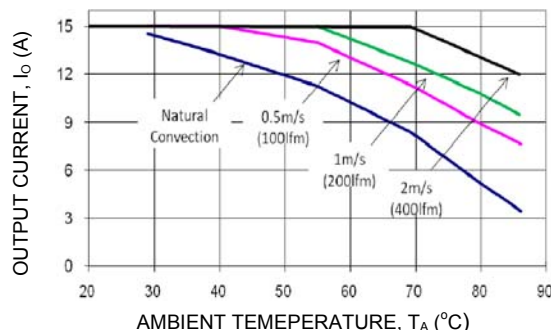
Figure 15. Output Current Derating for the Open Frame Module; Airflow in the Transverse Direction from V_{out}(-) to V_{out}(+) ; V_{IN} = 48V , V_O = 5.0V .
