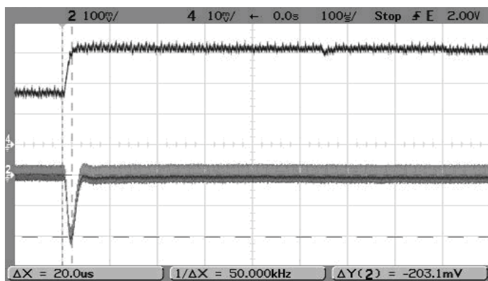
Step Load Transient Response (Vin=12V, Vout=5V, Clload=0, Iout=3A to 6A)
