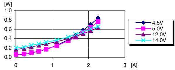
Dissipated power vs. load current and input voltage at T ref = +25°C
