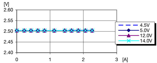
Output voltage vs. load current at T ref = +25°C
