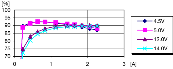
Efficiency vs. load current and input voltage at T ref = +25°C
