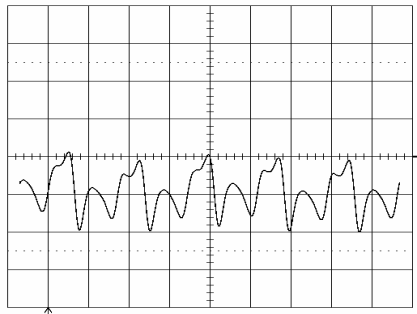
Output voltage ripple (20mV/div.) at: T_{ref} = +25^\circ\text{C} , I_O = 30\text{ A} resistive load, V_i = 5.0\text{ V} . Time scale: 2 \mu\text{s} /div. See the filter in the Output ripple and noise section (EMC Specification).
