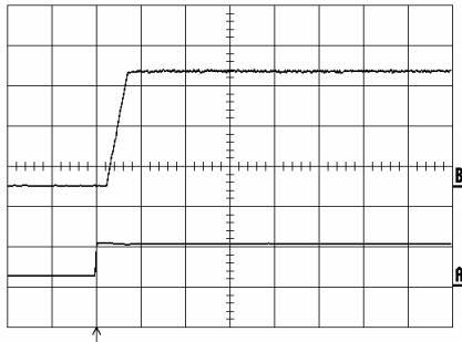
Start-up enabled by connecting V_i at: T_{ref} = +25^\circ\text{C} , I_O = 30\text{ A} resistive load, V_i = 5.0\text{ V} . Top trace: output voltage (0.5 V/div.). Bottom trace: input voltage (5 V/div.). Time scale: 10 ms/div..
