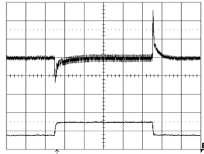
Output voltage response to load current step- change (15-30-15 A) at: T_{ref} = +25^\circ\text{C} , V_i = 5.0\text{ V} . Top trace: output voltage (100mV/div.). Bottom trace: load current (20 A/div.). Time scale: 0.1 ms/div..
