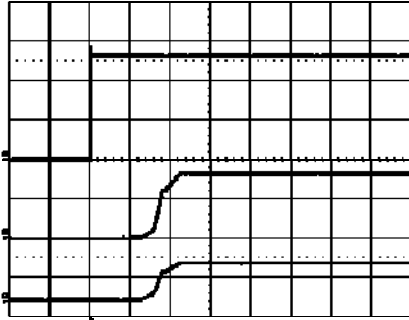
Start-up enabled by connecting V_i at: T_{ref} = +25^\circ\text{C} , V_i = 53\text{ V} , I_{o1} = 2.1\text{ A} , I_{o2} = 0.5\text{ A} resistive load. Bottom trace: output voltage 2 (5.0 V/div.). Mid trace: output voltage 1 (2.0 V/div.). Top trace: input voltage (20 V/div.). Time scale: (2 ms/div.).
