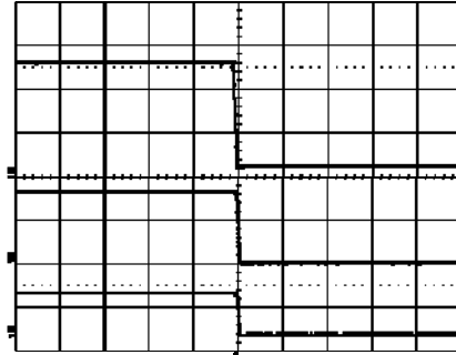
Shut-down enabled by disconnecting V_i at: T_{ref} = +25^\circ\text{C} , V_i = 53\text{ V} , I_{o1} = 2.1\text{ A} , I_{o2} = 0.5\text{ A} resistive load. Bottom trace: output voltage 2 (5.0 V/div.). Mid trace: output voltage 1 (2.0 V/div.). Top trace: input voltage (20 V/div.). Time scale: (2 ms/div.).
