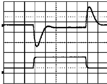
Output voltage response to load current step-change, output 1 (0.525-1.575-0.525 A) at: T_{ref} = +25^\circ\text{C} , V_i = 53\text{ V} , I_{o2} = 0.5\text{ A} . Top trace: output voltage 2 (100 mV/div.). Bottom trace: load current output 1 (1.0 A/div.). Time scale: (0.1 ms/div.).
