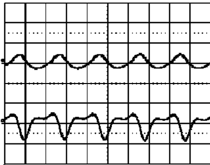
Output voltage ripple at: T_{ref} = +25^\circ\text{C} , V_i = 53\text{ V} , I_{o1} = 2.1\text{ A} , I_{o2} = 0.5\text{ A} resistive load. Top trace: output voltage 1 (10 mV/div.). Bottom trace: output voltage 2 (20 mV/div.). Time scale: (1 \mu\text{s} /div.).
