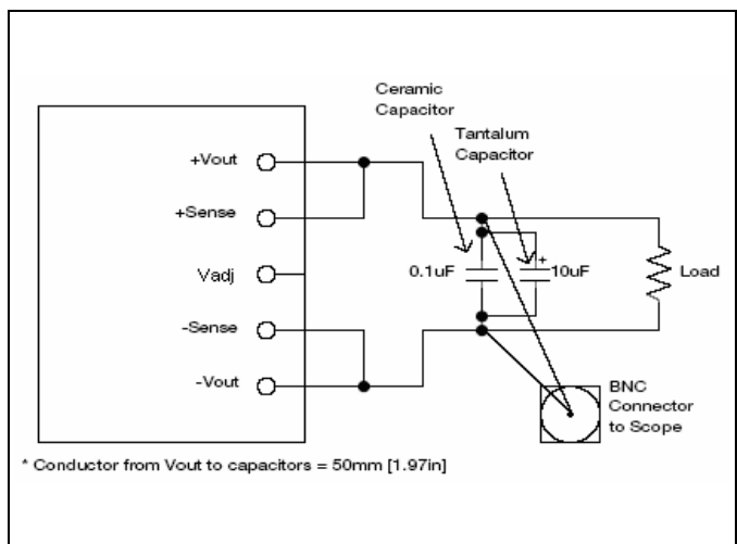
Output ripple and noise test setup
