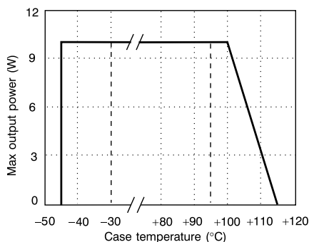
Power derating
