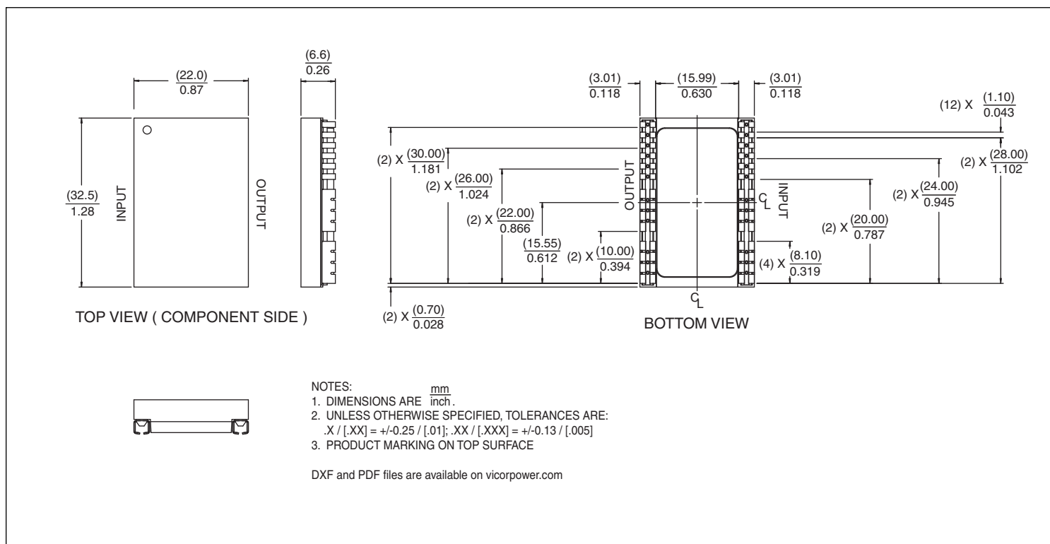
Figure 19 — PRM J-Lead mechanical outline; Onboard mounting
