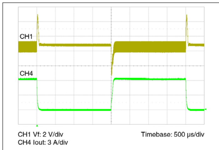
Figure 11 — Transient response; PRM alone 55 Vin, 0-6.7-0A no load capacitance, local loop
