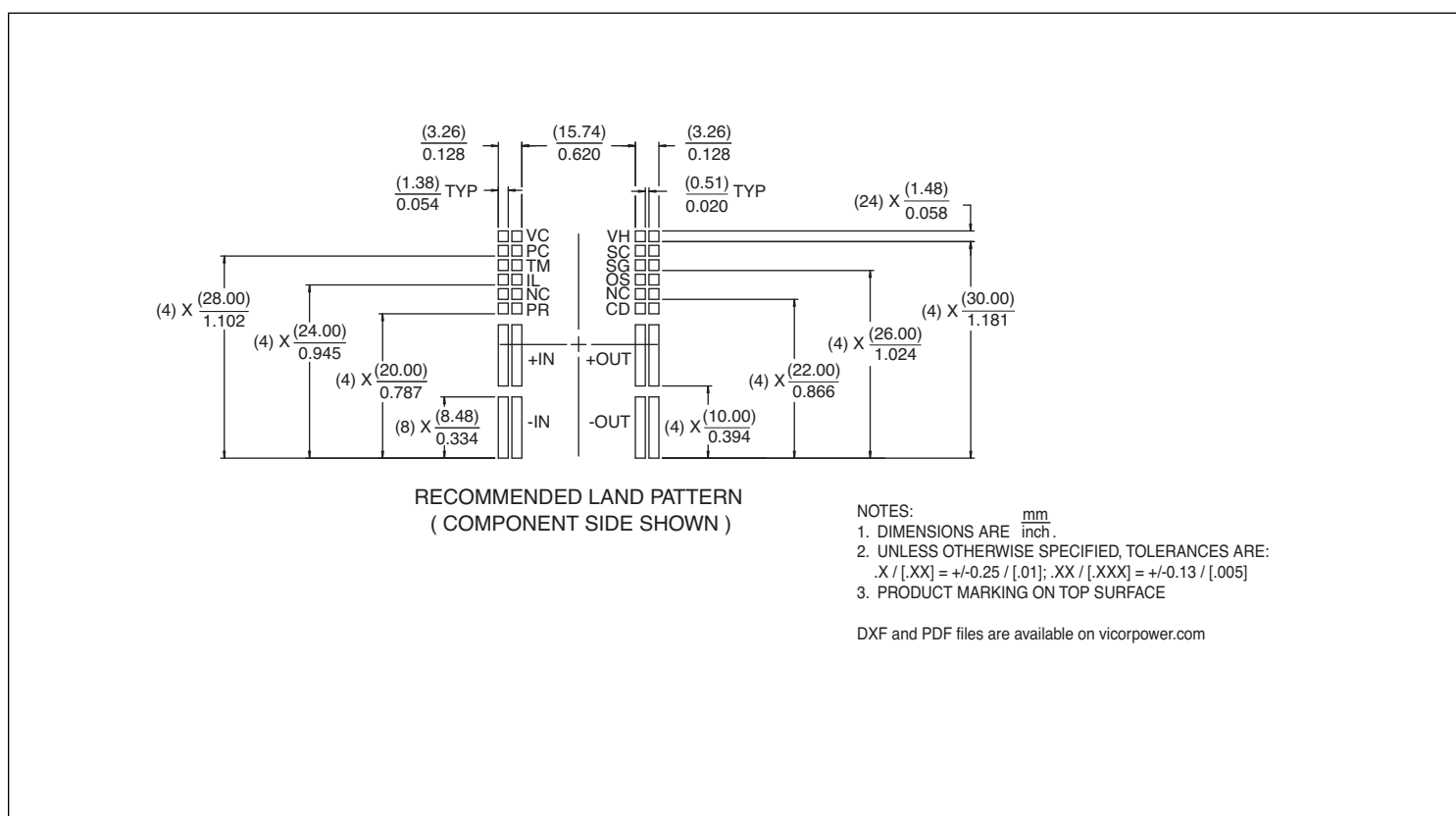
Figure 20 — PRM J-Lead PCB land layout information
