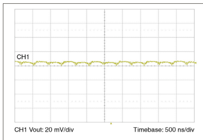
Figure 6 — Output voltage ripple at full load and 48 Vf with 47 \mu F ceramic POL bypass capacitance and 20 nH distribution inductance.
