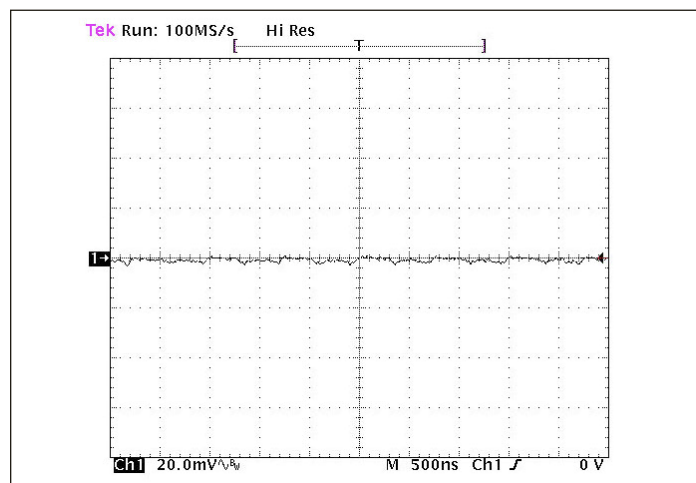
Figure 6 — Output voltage ripple at full load and 48 Vf with 100 \mu F ceramic POL bypass capacitance and 20 nH distribution inductance.
