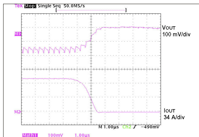
Figure 8 — 80.0-0 A load step with 100 \mu F input capacitance and no output capacitance.
