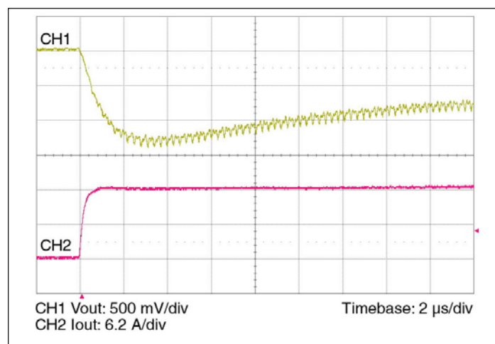
Figure 10 — 0-12.5 A load step with 100 \mu F input capacitor and no output capacitor.
