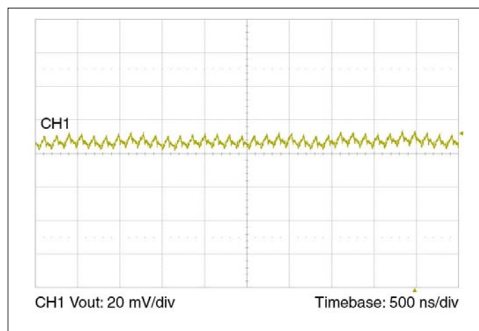
Figure 8 — Output voltage ripple at full load and 48 Vin with 3.3 \mu F ceramic external bypass capacitor and 20 nH of distribution inductance.
