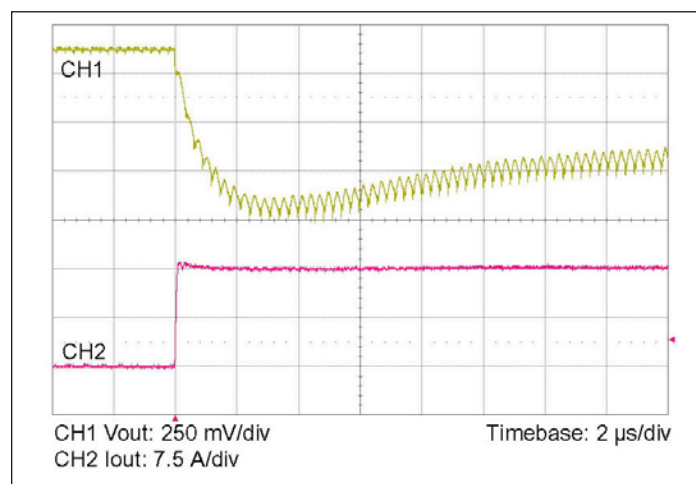
Figure 10 — 0-15 A load step with 100 \mu F input capacitor and no output capacitor.
