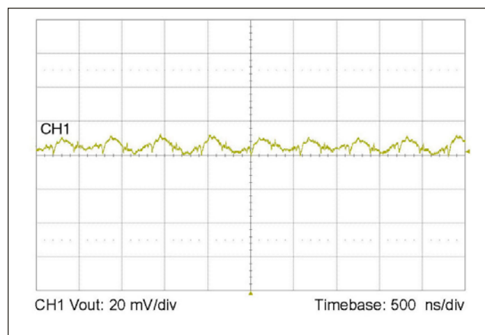
Figure 8 — Output voltage ripple at full load and 48 Vin with 10 \mu F ceramic external bypass capacitor and 20 nH of distribution inductance.
