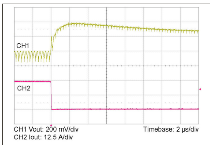
Figure 11 — 25-0 A load step with 100 µF input capacitor and no output capacitor.
