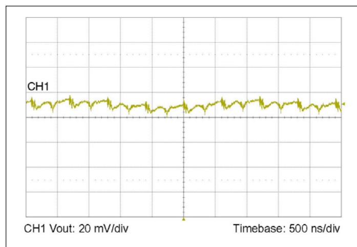
Figure 8 — Output voltage ripple at full load and 48 Vin with 10 µF ceramic external bypass capacitor and 20 nH of distribution inductance.
