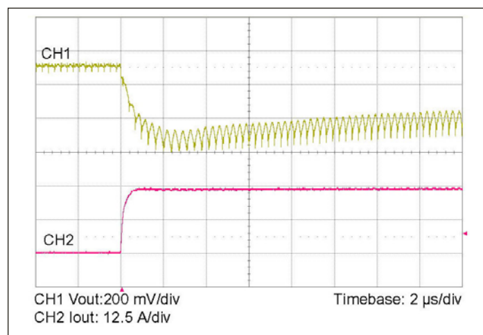
Figure 10 — 0-25 A load step with 100 µF input capacitor and no output capacitor.
