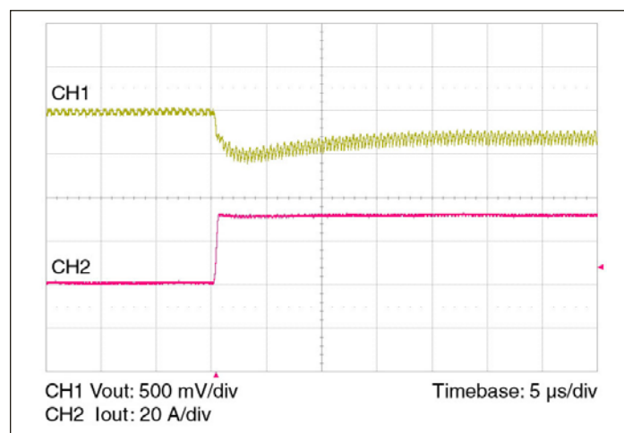
Figure 10 — 0-30 A load step with 100 \mu F input capacitor and no output capacitor.
