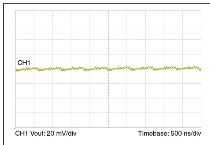
Figure 8 — Output voltage ripple at full load and 48 Vin with 30 \mu F ceramic external bypass capacitor and 20 nH of distribution inductance.
