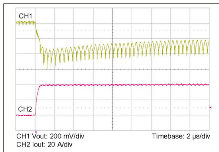
Figure 10 — 0-40 A load step with 100 \mu F input capacitor and no output capacitor.
