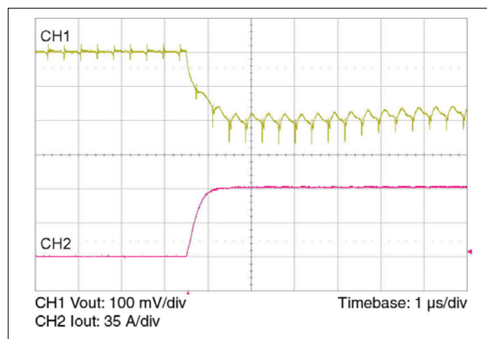
Figure 10 — 0-70 A load step with 100 µF input capacitor and no output capacitor.
