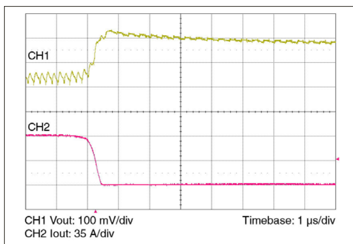
Figure 11 — 70-0 A load step with 100 µF input capacitor and no output capacitor.
