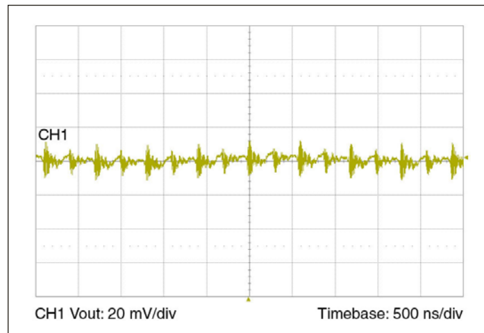
Figure 8 — Output voltage ripple at full load and 384 Vin with 10 µF ceramic external bypass capacitor and 20 nH of distribution inductance.
