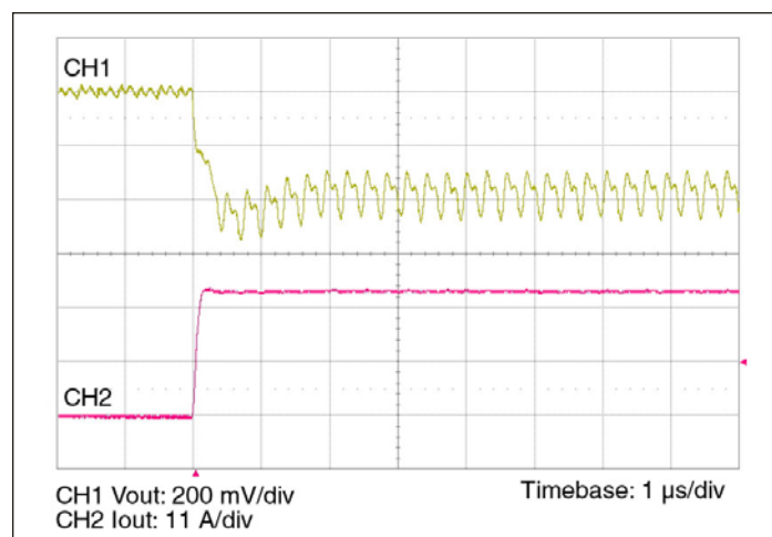
Figure 10 — 0-25 A load step with 2.2 µF input capacitor and no output capacitor.
