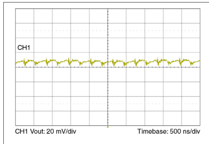
Figure 8 — Output voltage ripple at full load and 352 Vin with 10 \mu F ceramic external bypass capacitor and 20 nH of distribution inductance.
