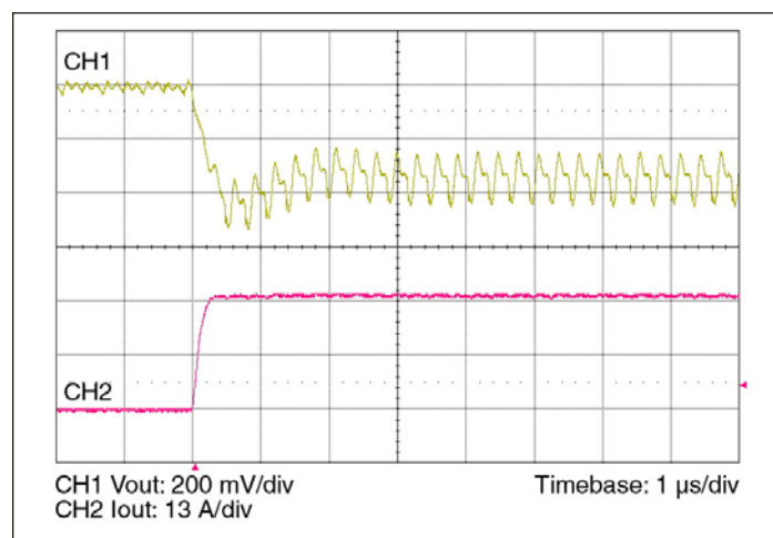
Figure 10 — 0-27.3 A load step with 2 \mu F input capacitor and no output capacitor.
