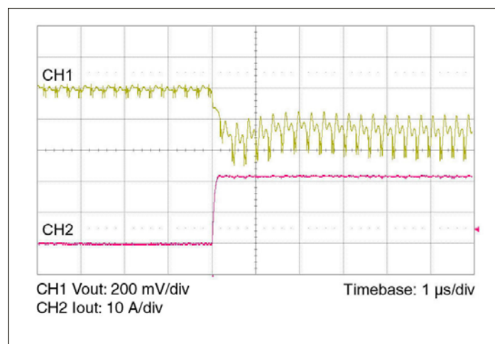
Figure 10 — 0-21.8 A load step with 2 µF input capacitor and no output capacitor.
