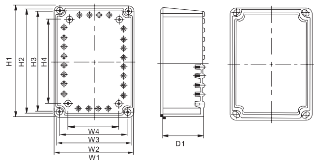
Dimension (Allowable error: ±1mm)
