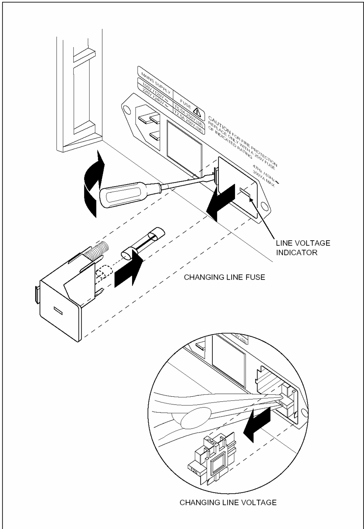
[图 2-1, 拆装保险丝和选择电源电压]
