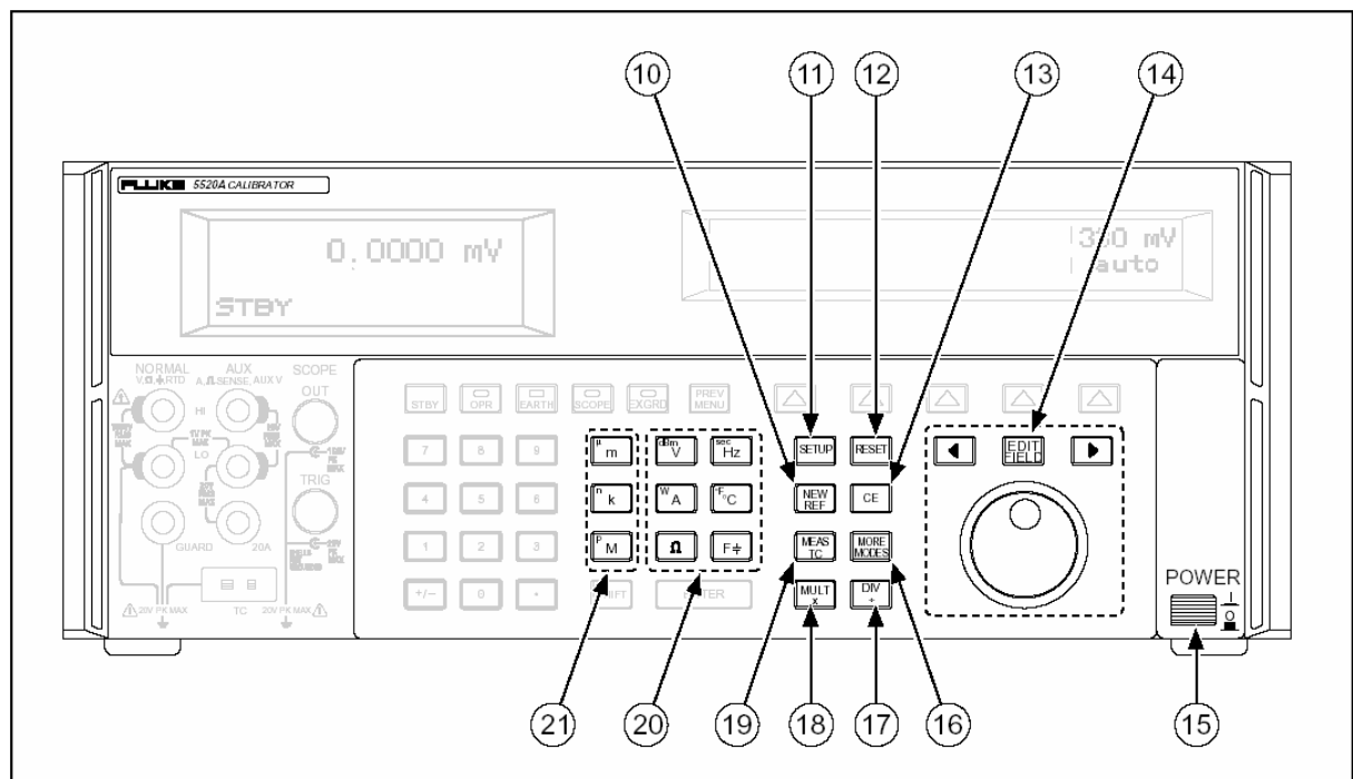
[图 3-1，前面板视图（续 1）]
