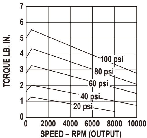
Torque vs. Speed
