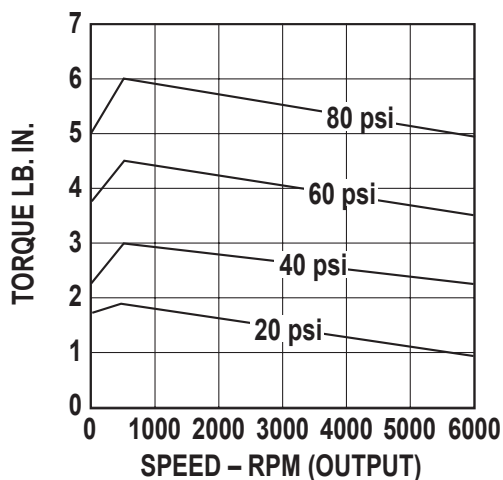
Torque vs. Speed
