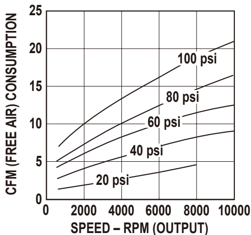
Air Consumption vs. Speed
