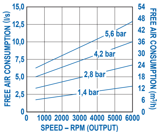
Air Consumption vs. Speed
