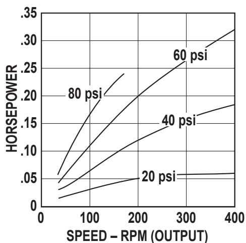
Output Power vs. Speed
