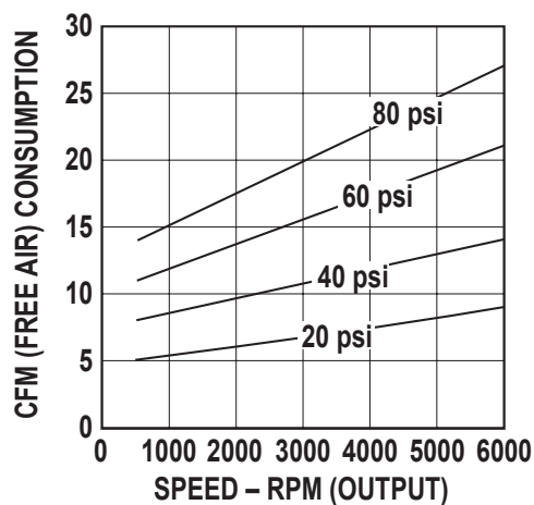
Air Consumption vs. Speed
