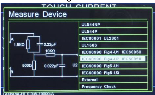
IEC60990 Fig4-U2、IEC60950
