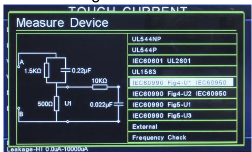
IEC60990 Fig4-U1、IEC60950
