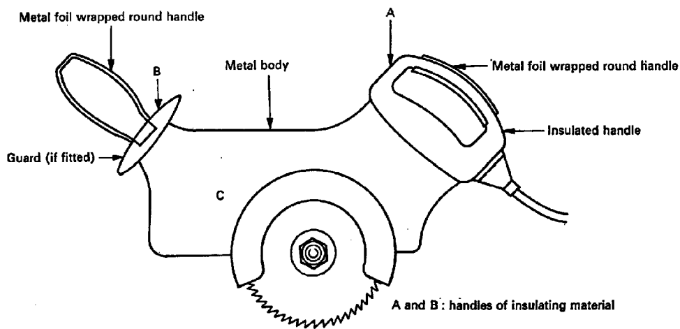
Figure 8c – Portable electric saw
