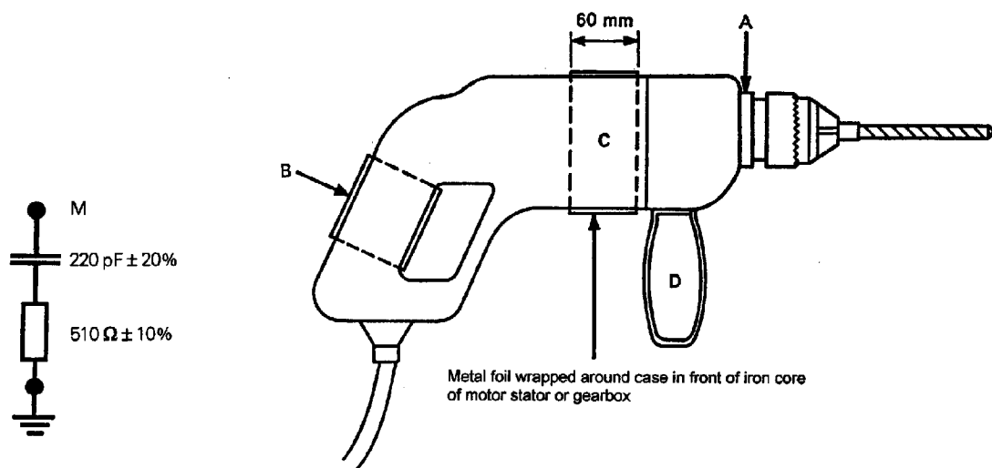
Figure 8a – RC element
