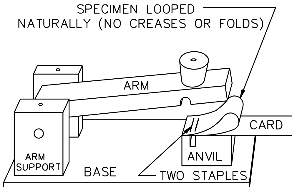
Figure 16.1 Specimen and arm in place before impact
