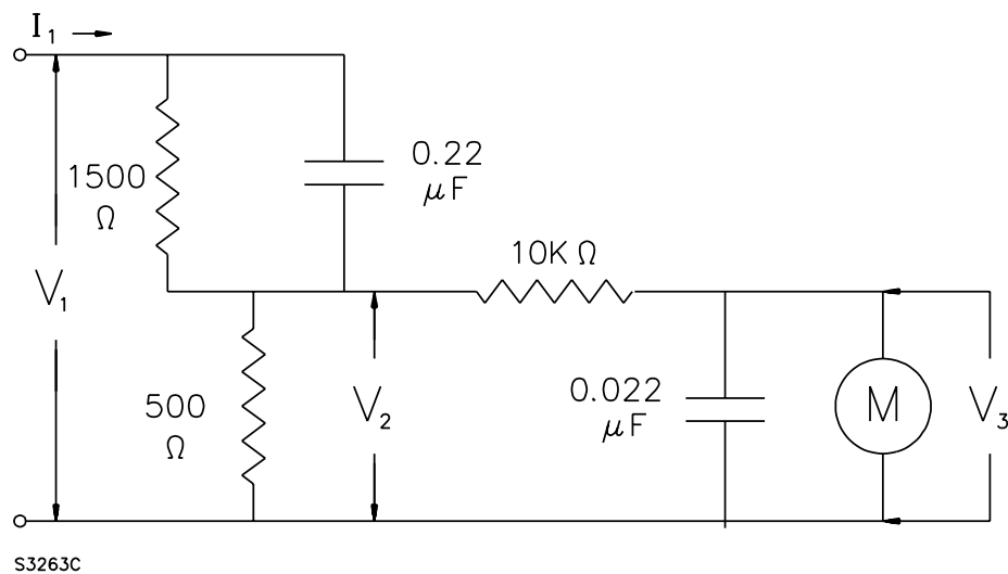
Figure 47.2 Measurement instrument for reaction (leakage) current
