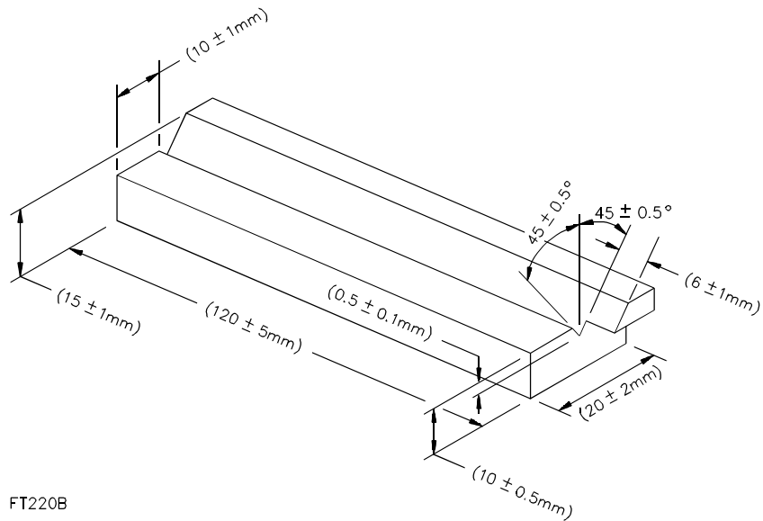
Figure 7.2 Flexible specimen support fixture
