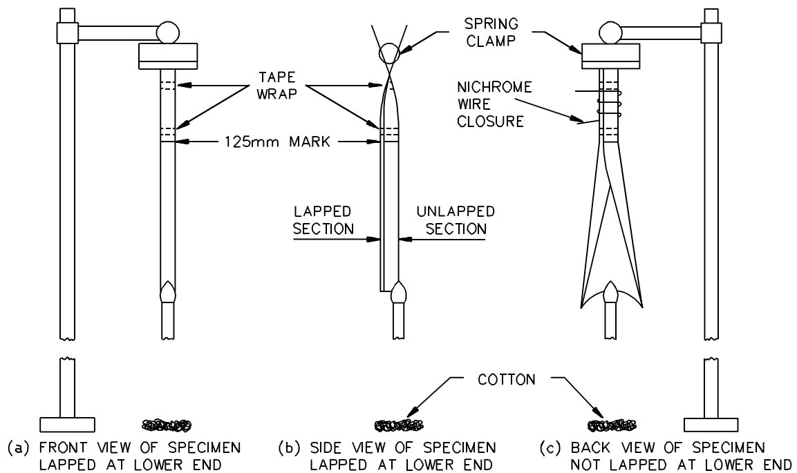
Figure 11.1 Specimen orientation
