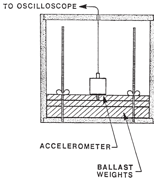
FIG. 2 Test Block
