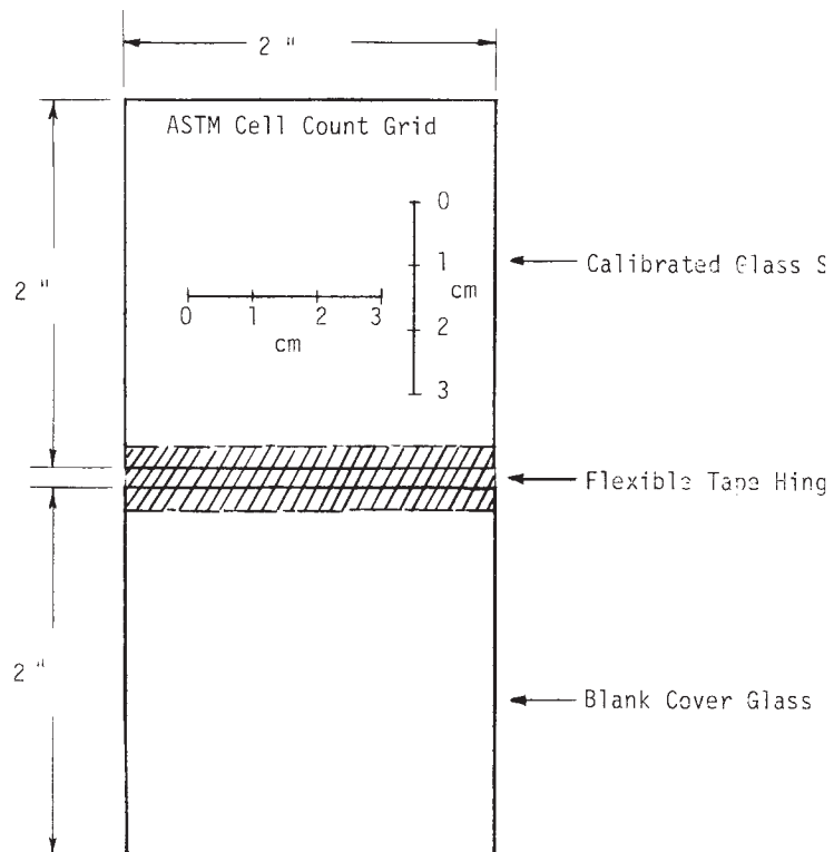
FIG. 2 Cell Size Scale Slide Assembly
