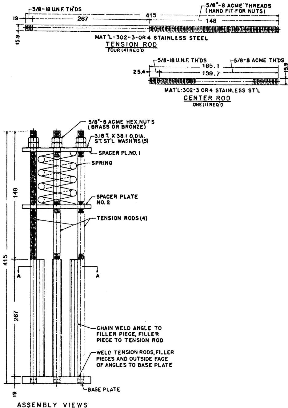
FIG. 2 Optional Compression-Type Deformation Tester
