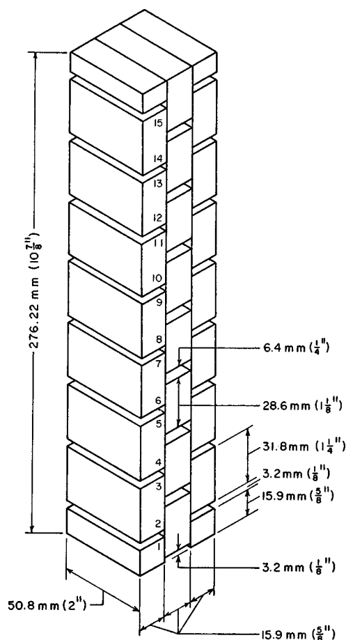
FIG. 3 View of Assembled Test Blocks
