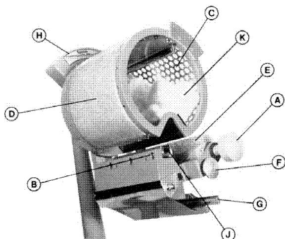
FIG. 1 Fibrosampler
