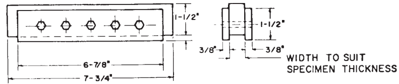
SPECIMEN LOADING BLOCKS 2 REQ'D
