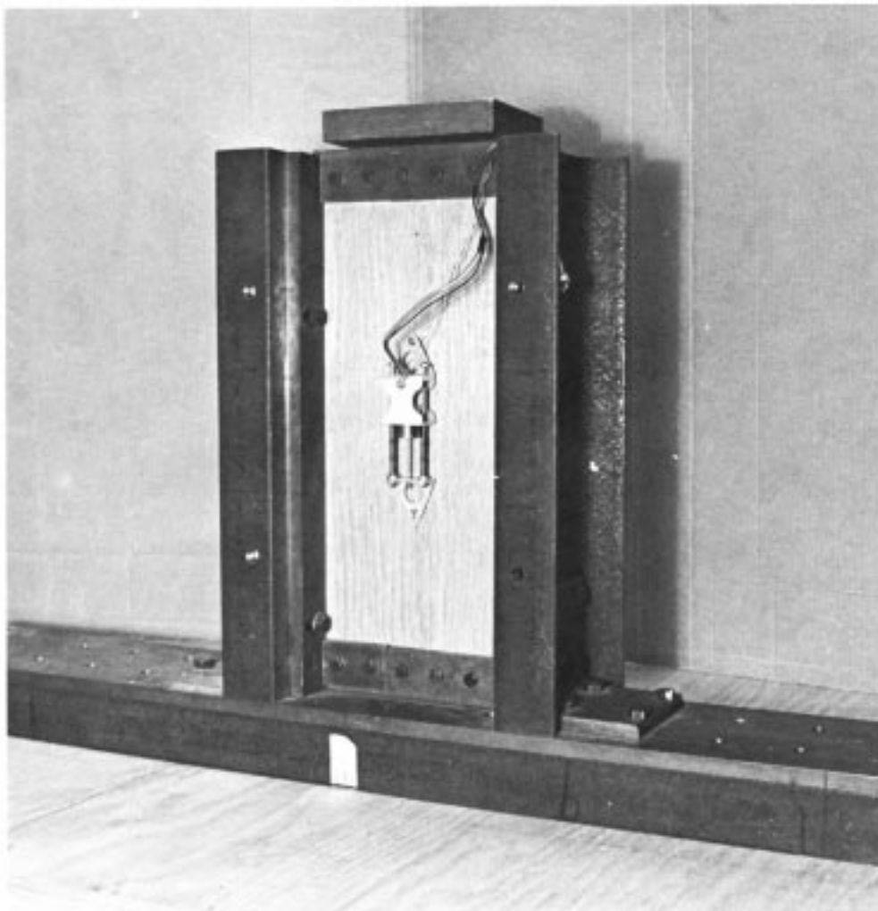
FIG. 5 Method B, Loading Hardware Showing a Specimen Mounted with Transducers for Deformation Measurement
