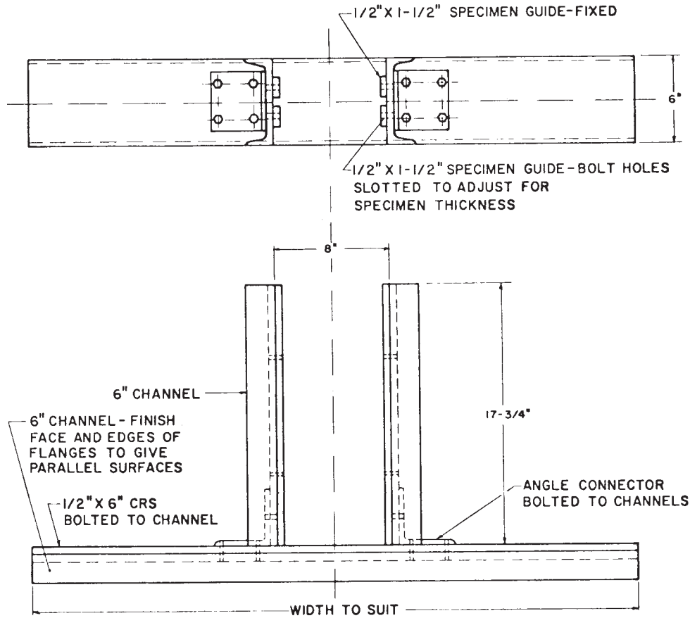
SPECIMEN LOADING BLOCKS 2 REQ'D
