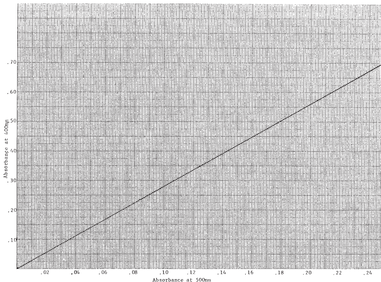
FIG. 1 Correction Graph
