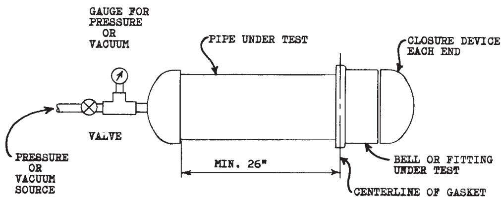
FIG. 1 Test Specimen
