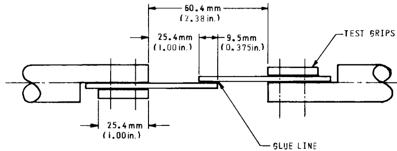
FIG. 1 Test Specimen
