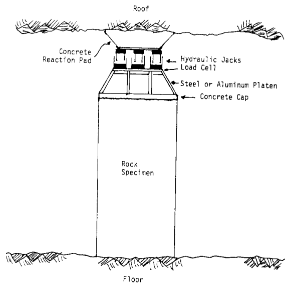
FIG. 2 Test Arrangement
