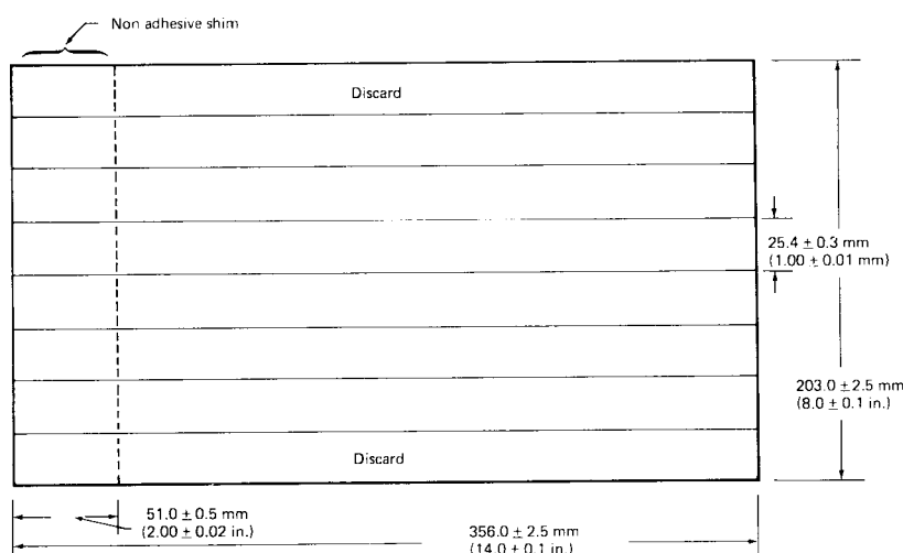
FIG. 2 Test Joint
