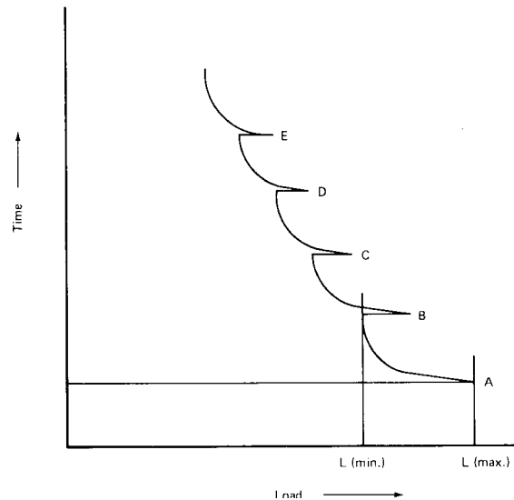
FIG. 4 Typical Flat Adherend Test
