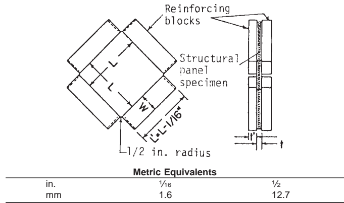
FIG. 1 Small Panel Shear Specimen and Dimensions
