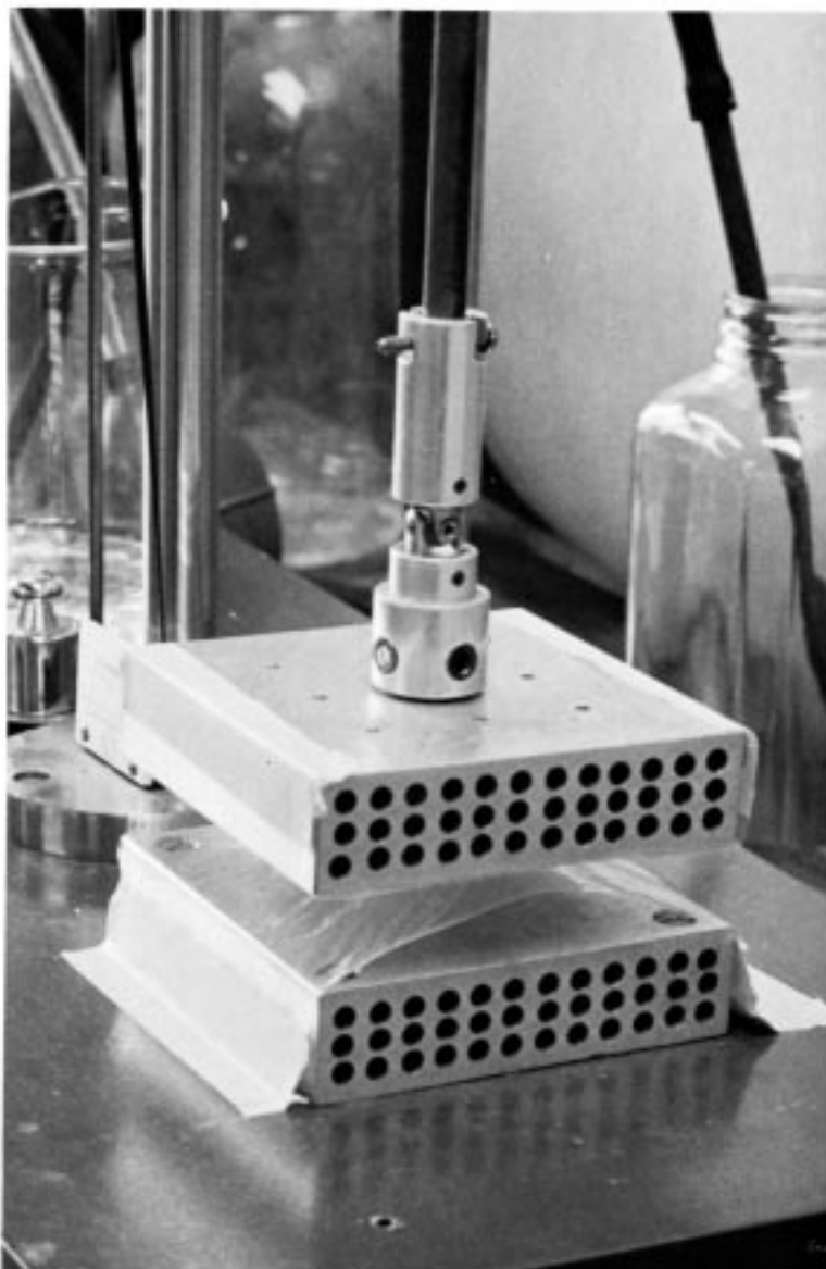
FIG. 3 Suspended and Stationary Aluminum Blocks
