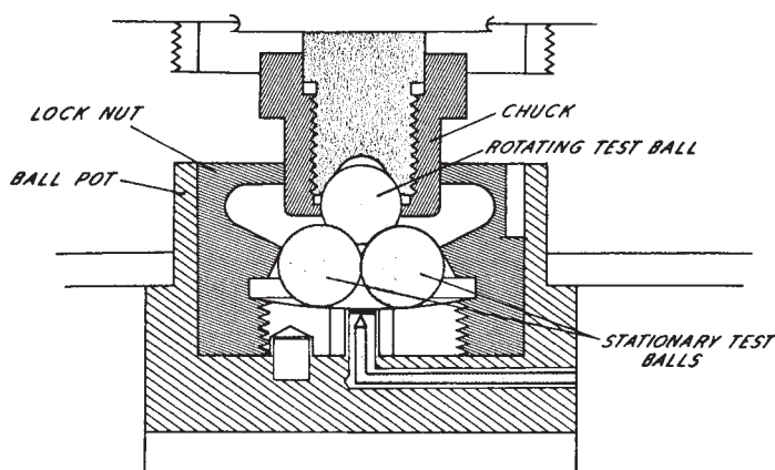
FIG. 2 Falex Corporation (Roxanna) Four-Ball Test Arrangement
