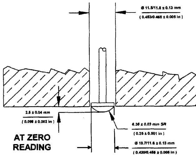
FIG. 1 (e) Type OOO Indenter (continued)
