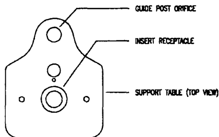
FIG. 2 Durometer Operating Stand
