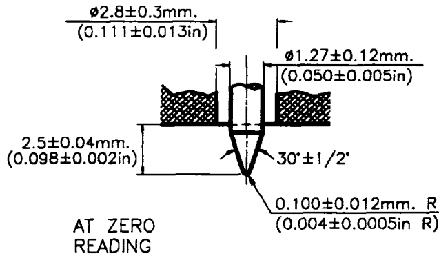
FIG. 1 (b) Type B and D Indentor (continued)
