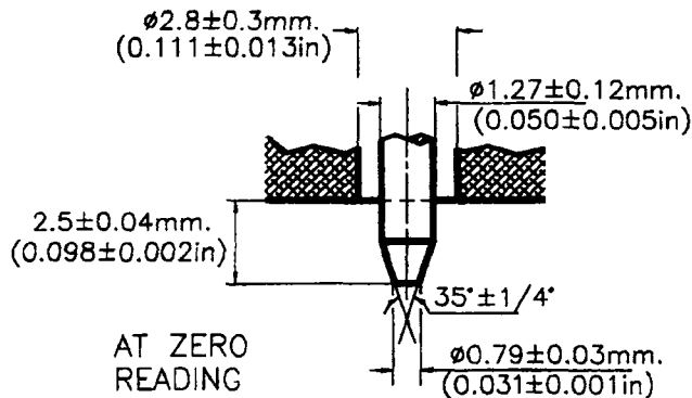
FIG. 1 (a) Type A and C Indenter
