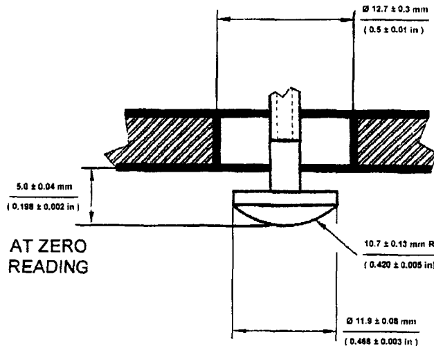
FIG. 1 (f) Type OOO-S Indenter (continued)
