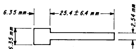
FIG. 2 Modified T-50 Test Piece
