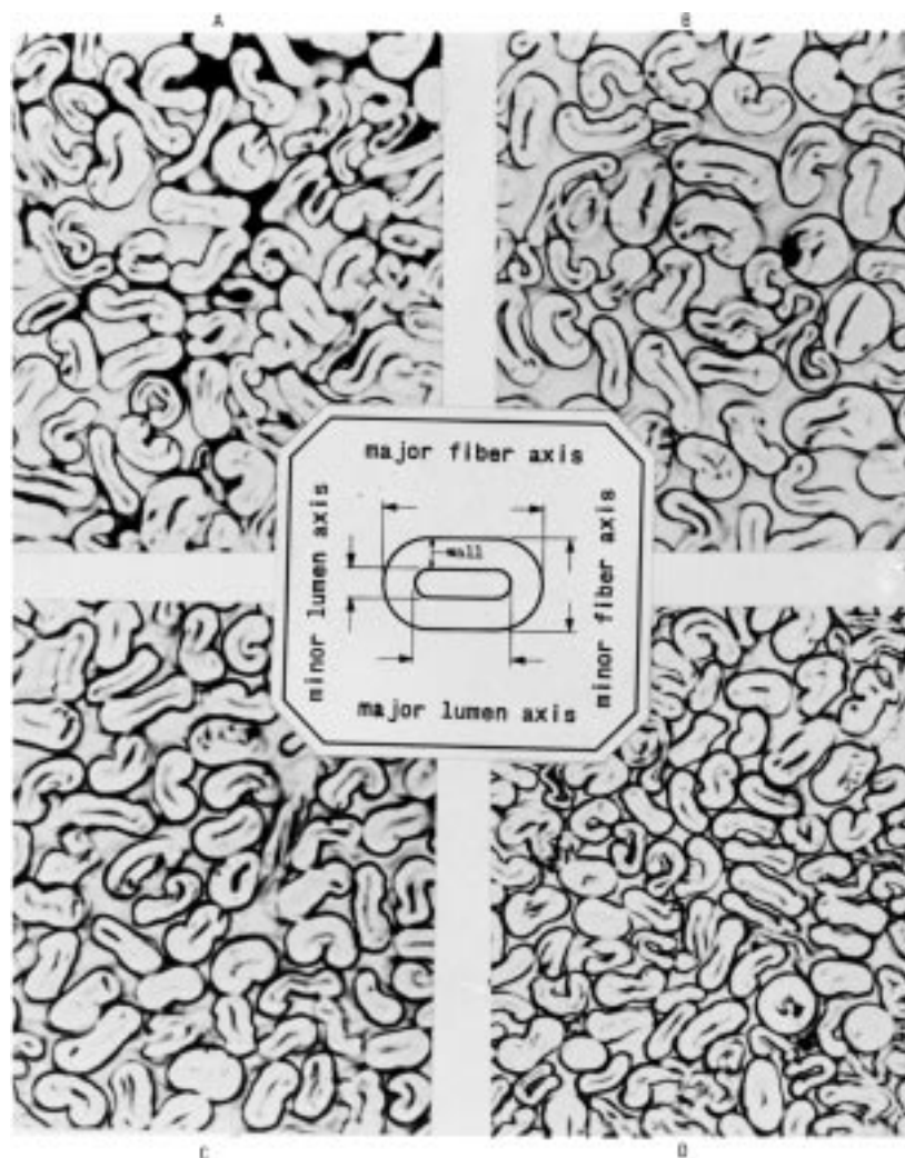
FIG. A1.1 Representative Cross Sections of Different Varieties of Cotton (magnification approx 625x)
