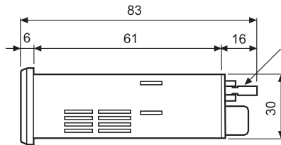
<MT4Y-□□-45>
